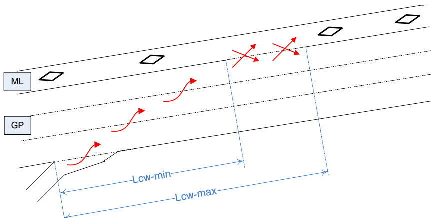
FIGURE 4.13 Defining Dimensions of APIA through Minimum and Maximum Cross-Weave Lengths
