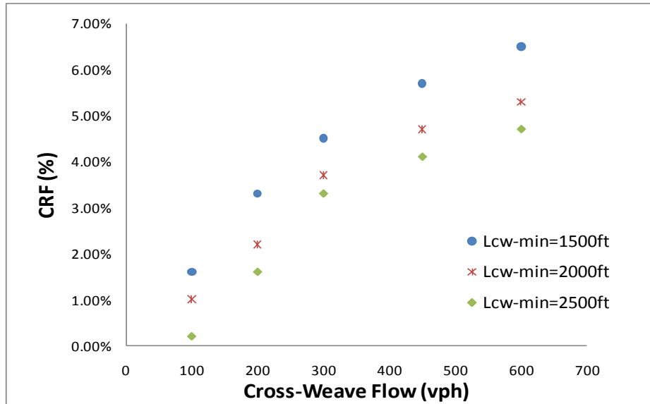
FIGURE 5.16 CRF as Response to Cross Weave Flow and Lcw-min under 4-Lane GP Scenarios
